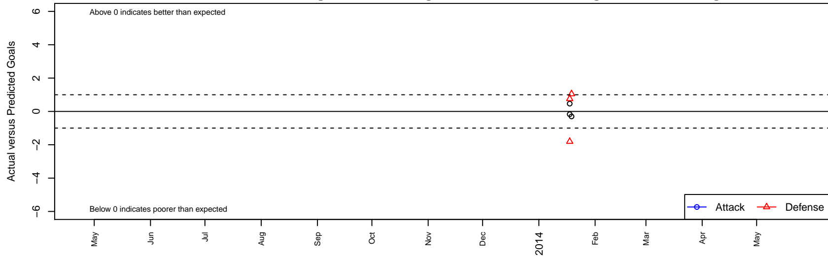
Irvine Slammers G01 Dots are actual minus expected GF (blue circles) and GA (red triangles). Blue line is smoothed change in attack strength. Red is smoothed change in defense strength.
